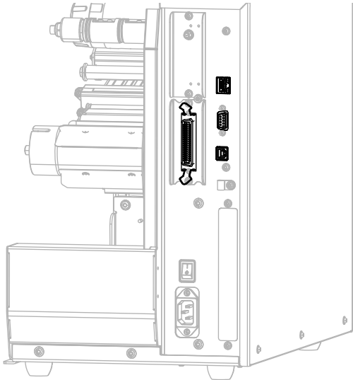
Figure 17 Location of Communication Interfaces
