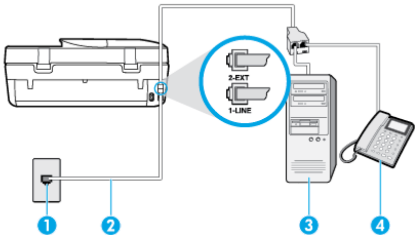
Figure B-18 Back view of the printer
