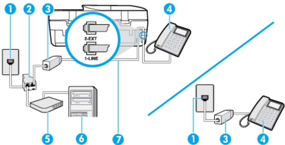
Figure B-10 Back view of the printer
