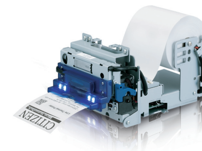
PMU2300III without presenter
